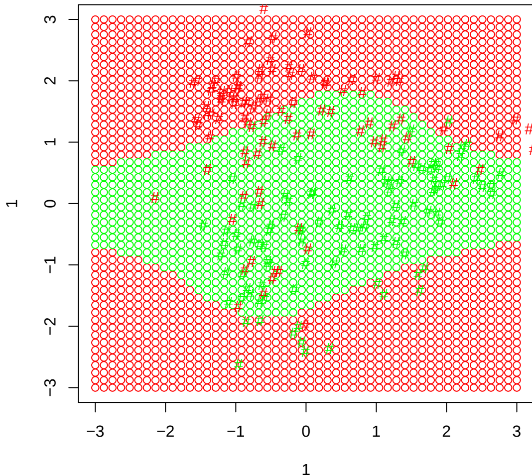
Polyn. kernel, degree 4, gamma = 100
