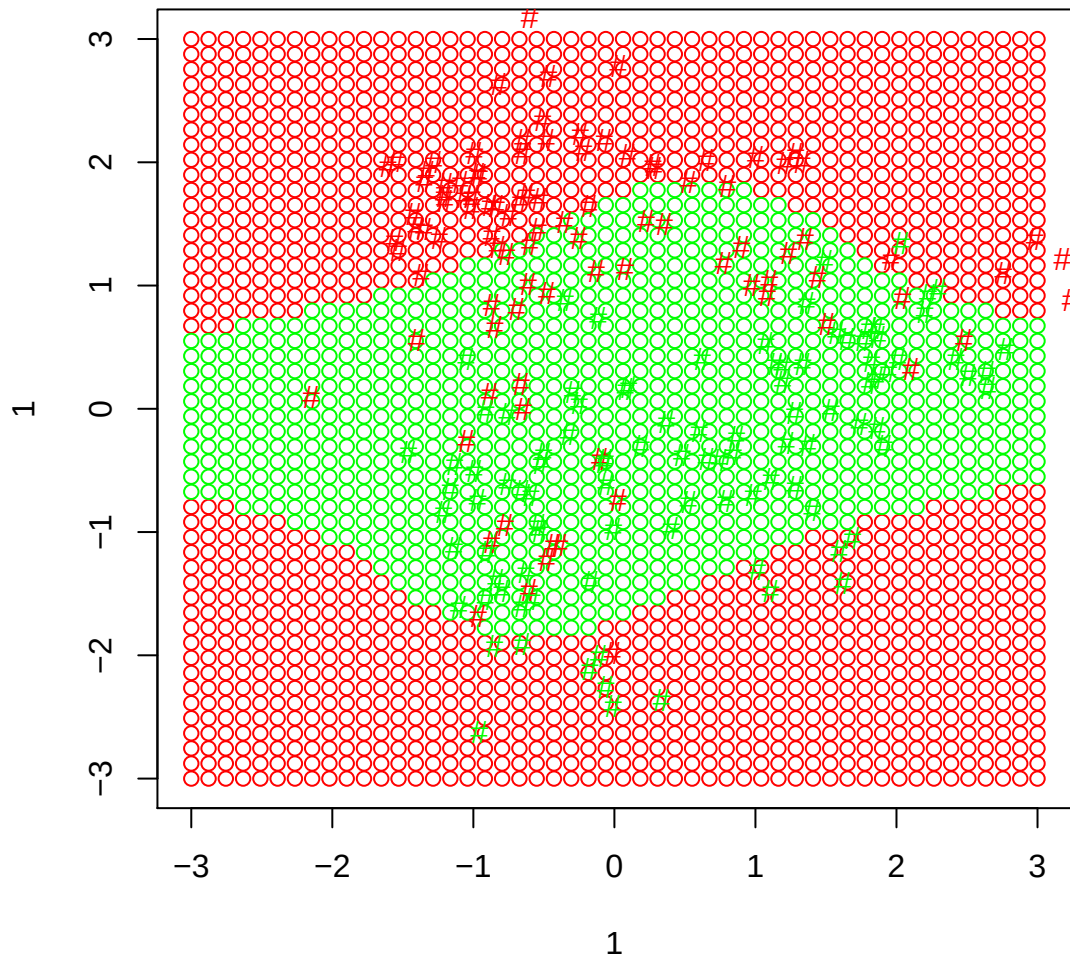
Polyn. kernel, degree 4, gamma = 1
