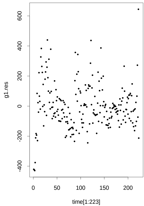
Figure 2: Second degree polynomial fit and the residuals plot for Casey data.
