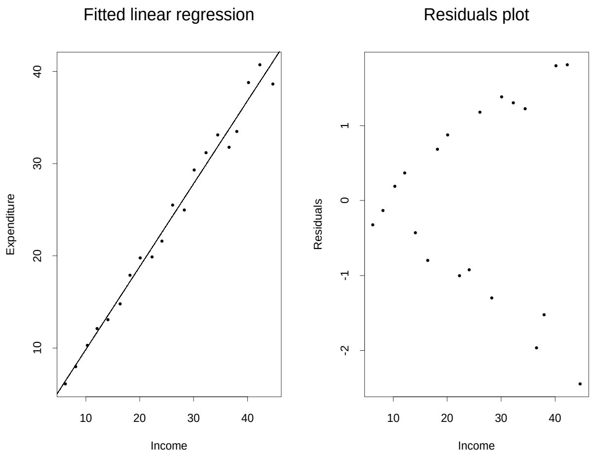
Figure 1: Heteroscedasticity in parametric linear regression.
