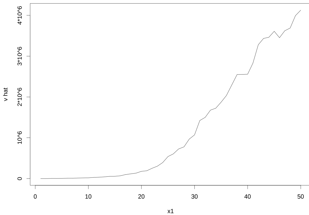
Figure 7: Variance function for simulated data.
