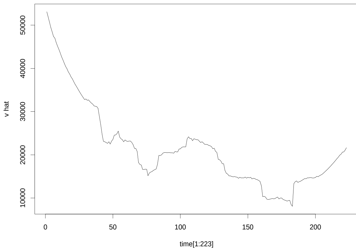
Figure 3: Variance function for Casey data.
