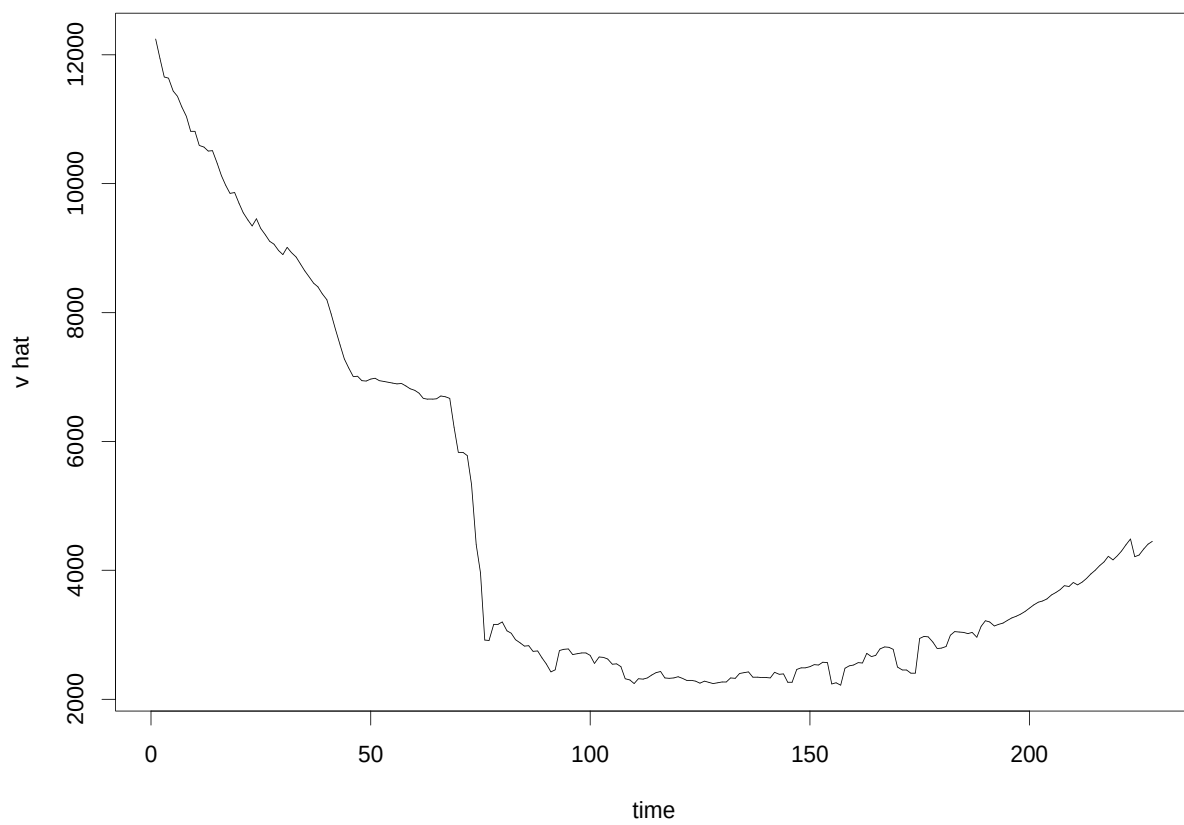
Figure 5: Variance function for Hudson data.
